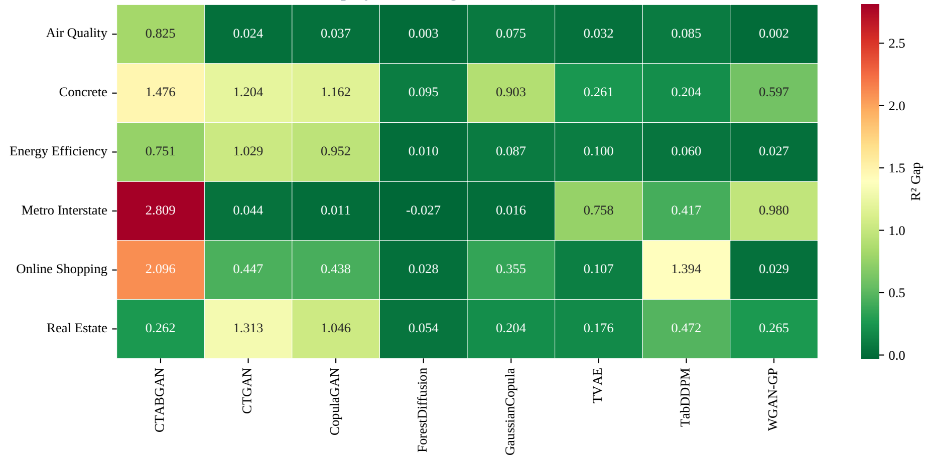
R 2 Gap by dataset × generator (10-seed mean)
